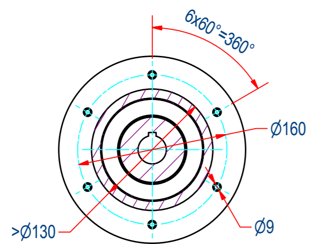
H-H MOUNTING DETAIL (2x) HOLE PATTERN COUNTER PART
