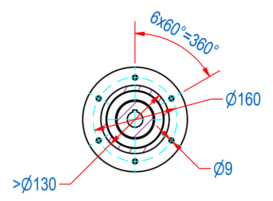
C-C MOUNTING DETAIL (2x) HOLE PATTERN COUNTER PART
