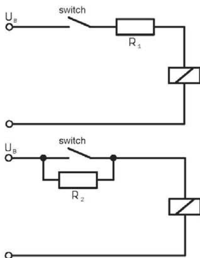
Example: Contact protection via a current-limiting resistance
