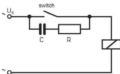
Example: Contact protection via an RC-circuit
