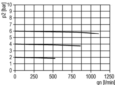
flow characteristic
