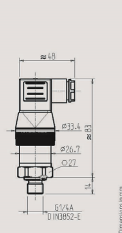
with angular connector DIN 175301-803 A and zero point adjustment
