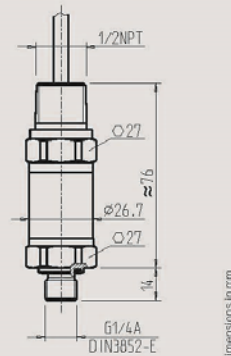
with cable outlet 1/2 NPT conduit
