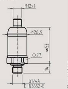
with M12 x 1 circular connector (4-pin, metallic)
