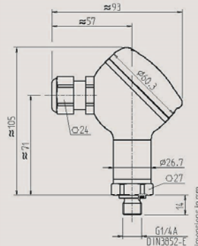
with field case
