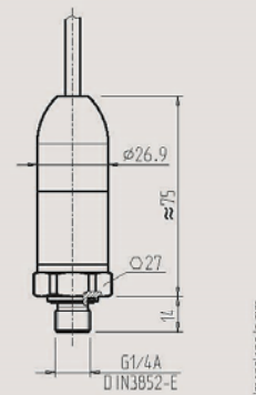
with cable outlet IP 68, FER, IP 6K9K
