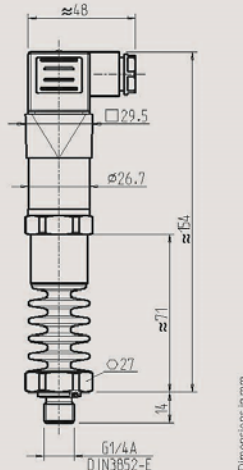
with angular connector DIN 175301-803 A and cooling element
