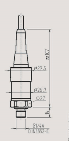
with cable outlet IP 67
