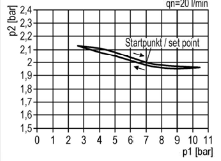
pressure characteristic
