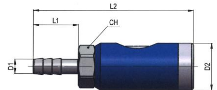
Hose stem
