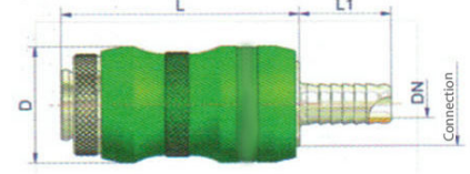
Hose connection
