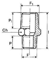
Double nipple, conical male thread
