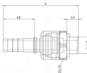
Hose stem, male
