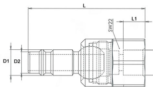
Plug, swivel type
