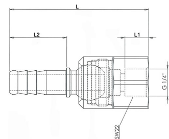
Hose stem, female
