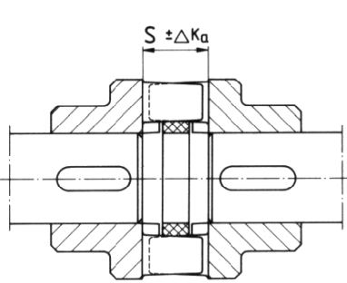
Fig. 2: Axial misalignment
