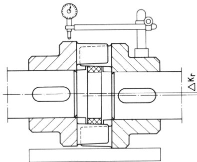
Fig. 3: Radial misalignment
