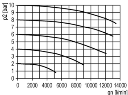
flow characteristic
